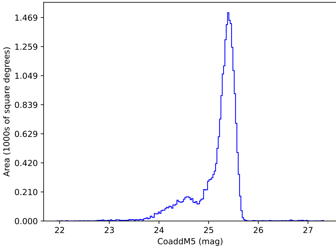
too_elab_r8_d3_gz_v3.4_10yrs u: CoaddM5
