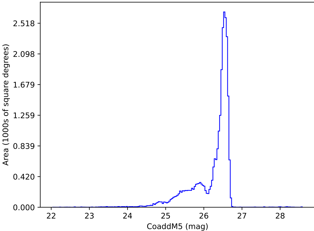
too_elab_r8_d3_gz_v3.4_10yrs i: CoaddM5
