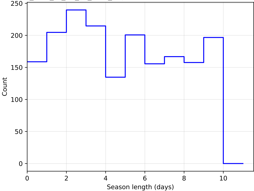
too_elab_r8_d3_gz_v3.4_10yrs DD:WFD all bands: SeasonLength
