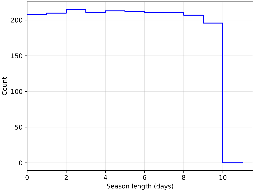
too_elab_r8_d3_gz_v3.4_10yrs DD:EDFS all bands: SeasonLength
