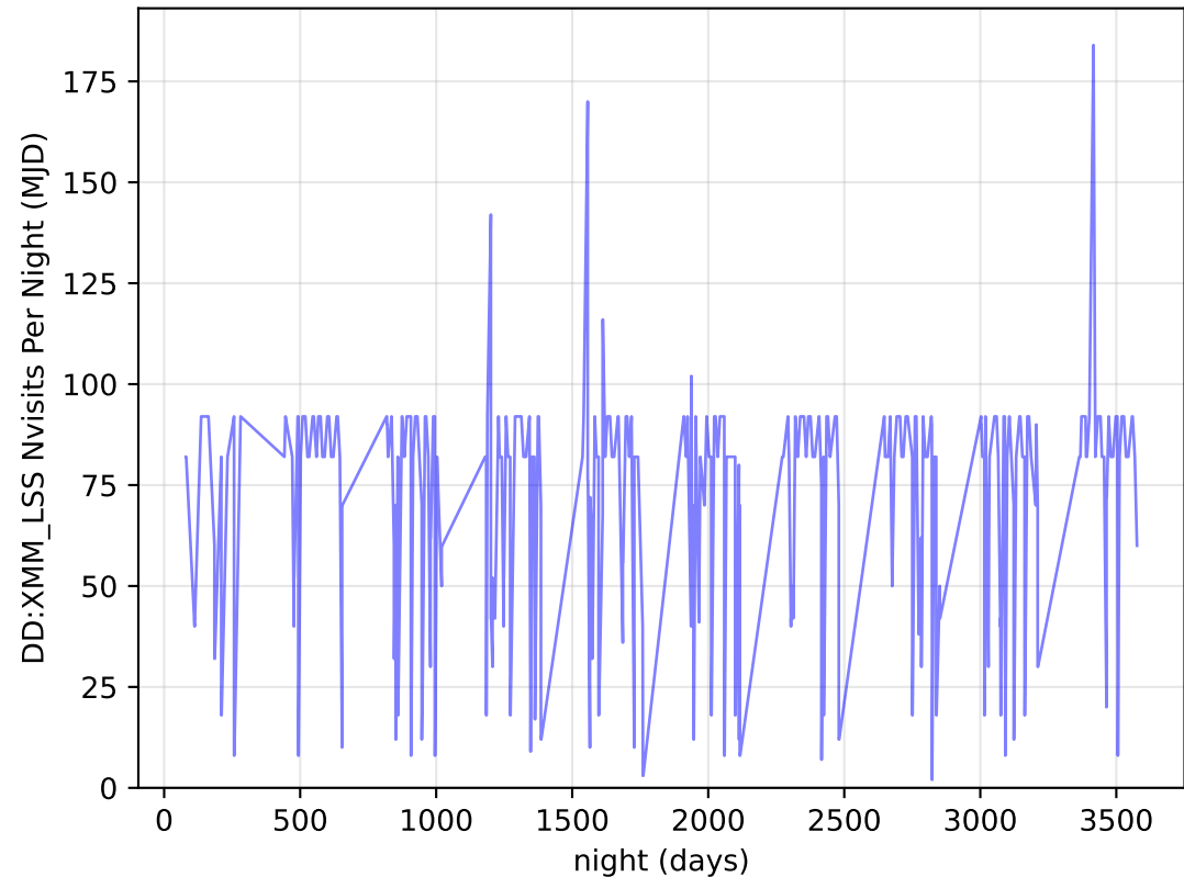
too_elab_r8_d3_gz_v3.4_10yrs all bands: DD:XMM_LSS Nvisits Per Night
