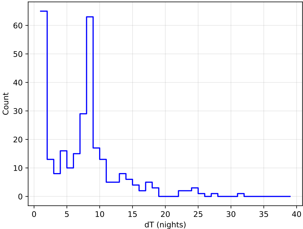
too_elab_r8_d3_gz_v3.4_10yrs all bands: DD:XMM_LSS Delta Nights Histogram
