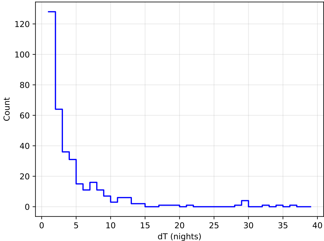
too_elab_r8_d3_gz_v3.4_10yrs all bands: DD:WFD Delta Nights Histogram
