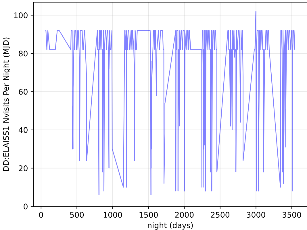
too_elab_r8_d3_gz_v3.4_10yrs all bands: DD:ELAISS1 Nvisits Per Night
