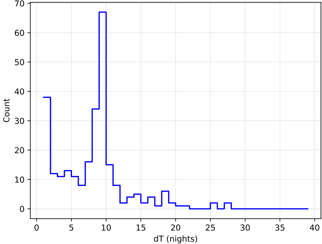
too_elab_r8_d3_gz_v3.4_10yrs all bands: DD:ELAISS1 Delta Nights Histogram
