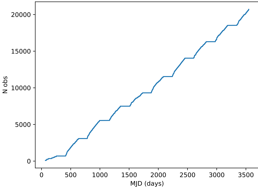
too_elab_r8_d3_gz_v3.4_10yrs all bands: DD:ELAISS1 Cumulative NVisits
