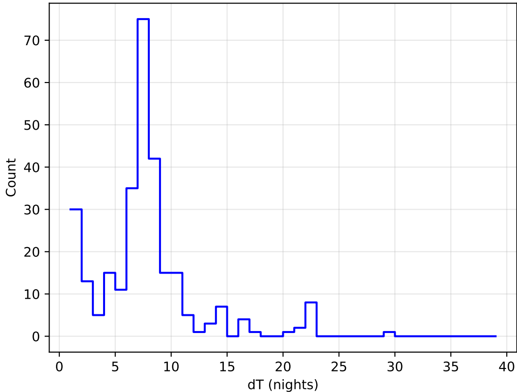
too_elab_r8_d3_gz_v3.4_10yrs all bands: DD:EDFS Delta Nights Histogram
