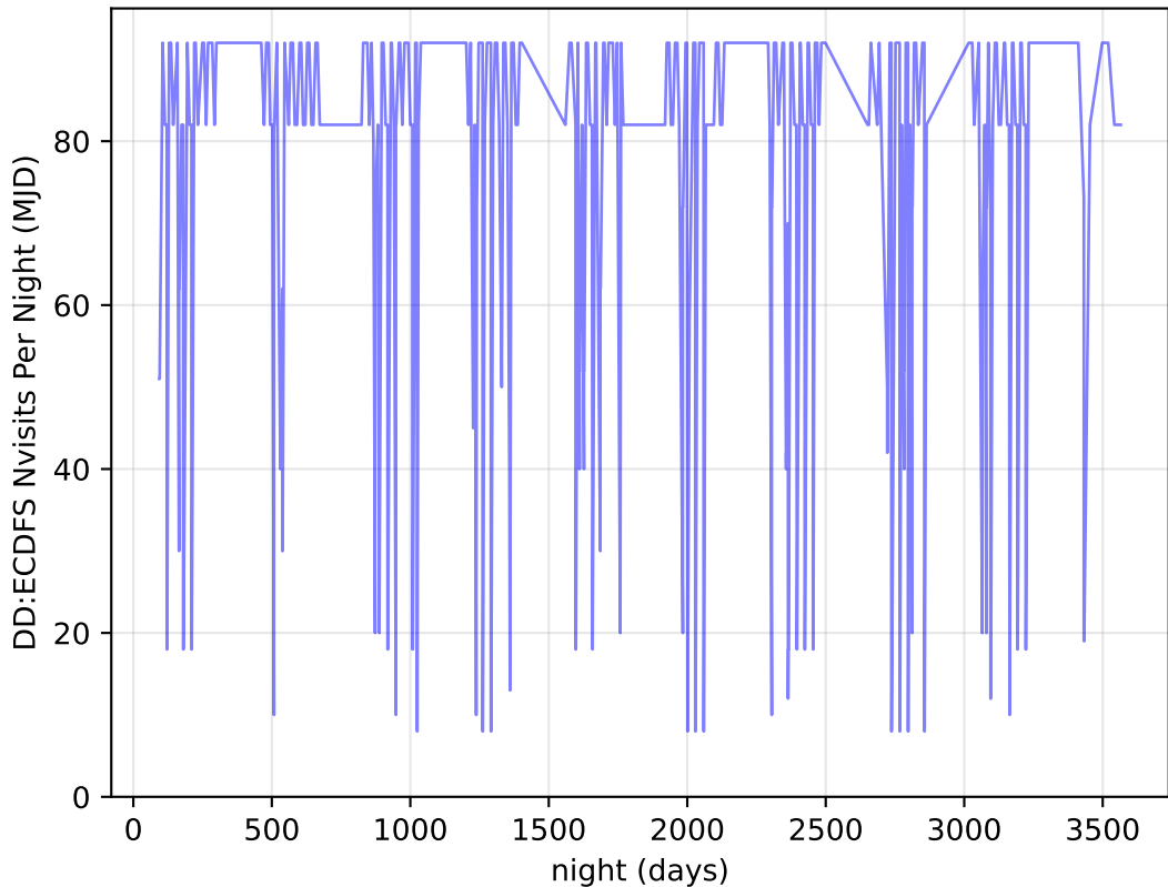
too_elab_r8_d3_gz_v3.4_10yrs all bands: DD:ECDFS Nvisits Per Night
