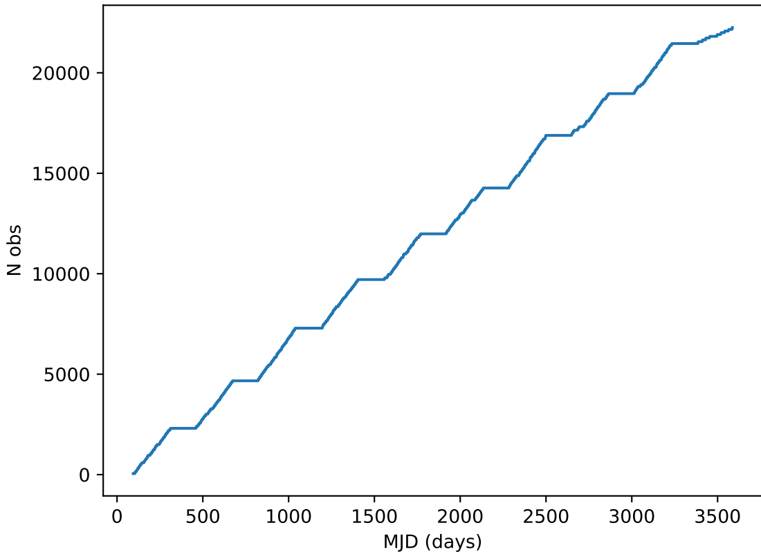
too_elab_r8_d3_gz_v3.4_10yrs all bands: DD:ECDFS Cumulative NVisits
