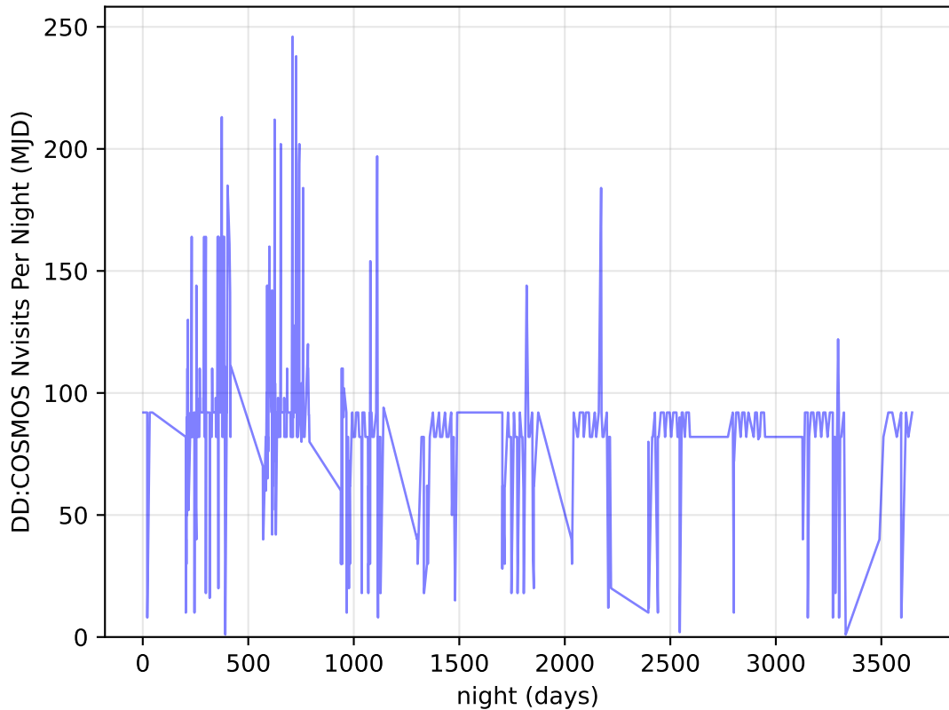
too_elab_r8_d3_gz_v3.4_10yrs all bands: DD:COSMOS Nvisits Per Night
