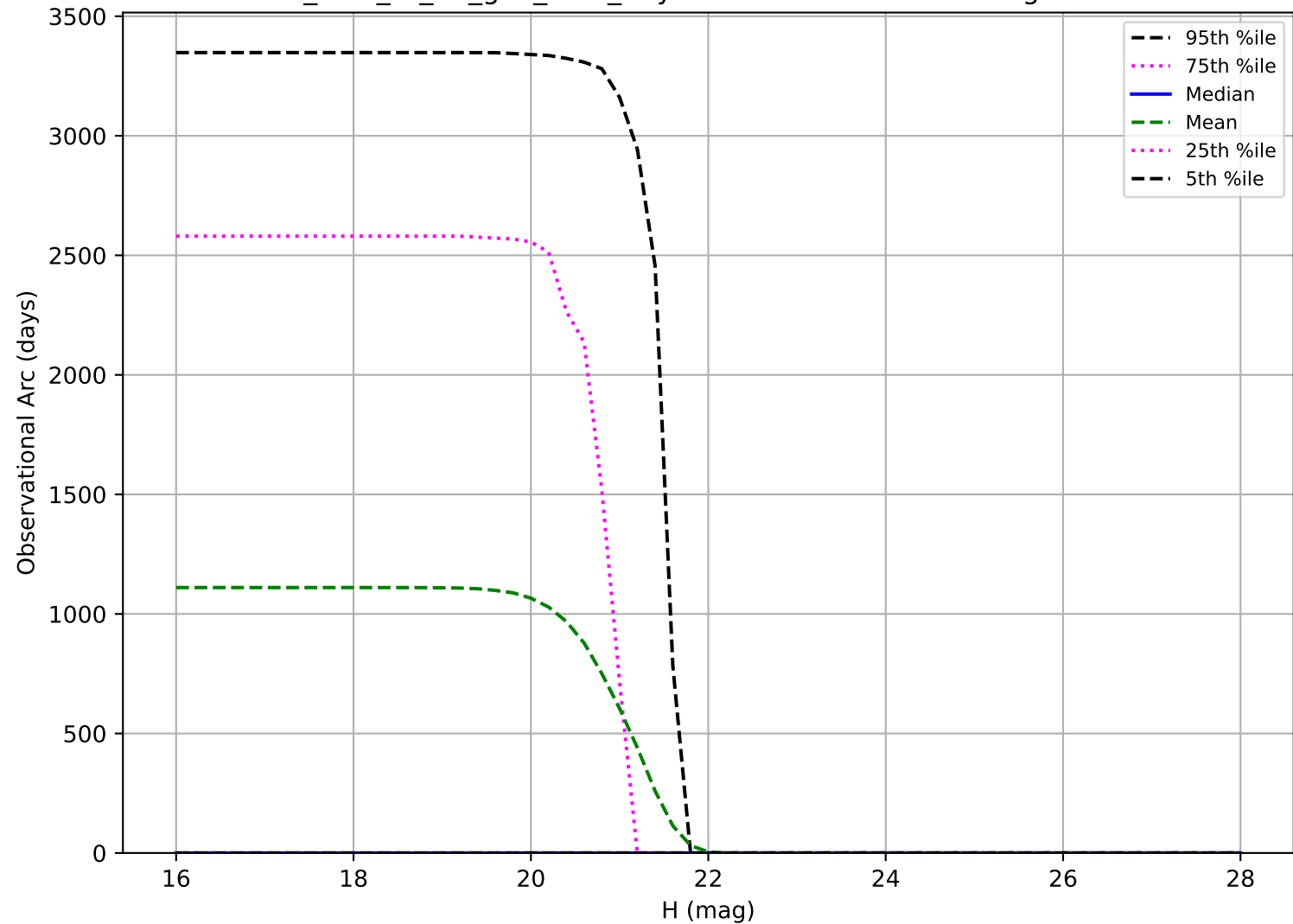
too_elab_r8_d3_griz_v3.4_10yrs: Observational Arc Length Vatira
