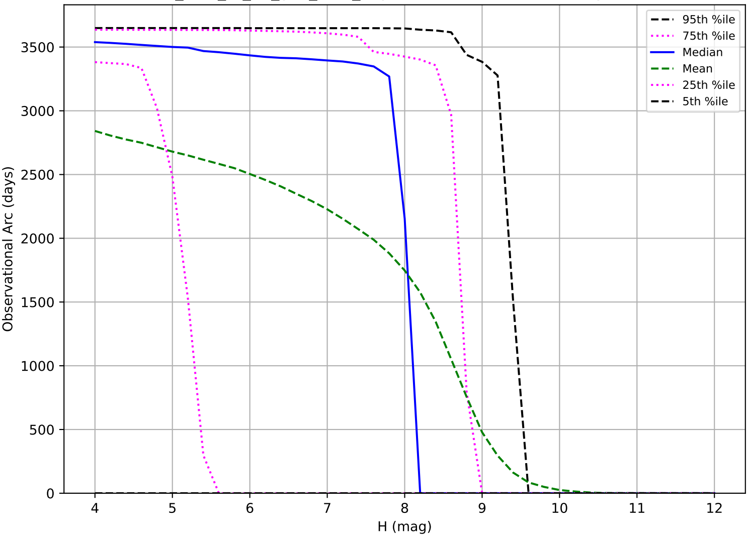
too_elab_r8_d3_griz_v3.4_10yrs: Observational Arc Length TNO
