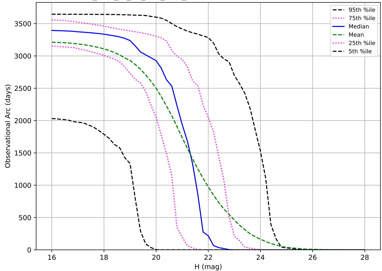
too_elab_r8_d3_griz_v3.4_10yrs: Observational Arc Length PHA
