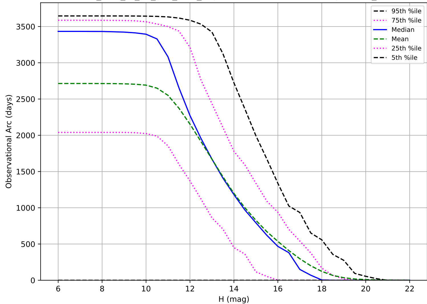
too_elab_r8_d3_griz_v3.4_10yrs: Observational Arc Length OCC_r5
