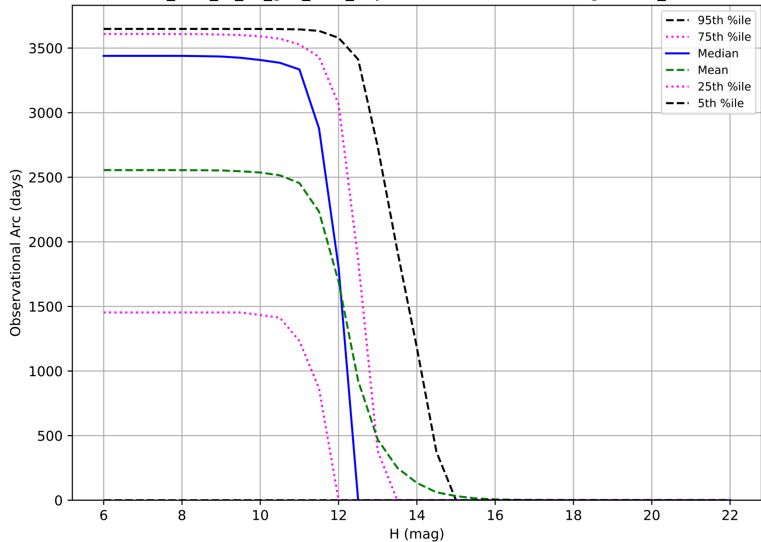
too_elab_r8_d3_griz_v3.4_10yrs: Observational Arc Length OCC_r20
