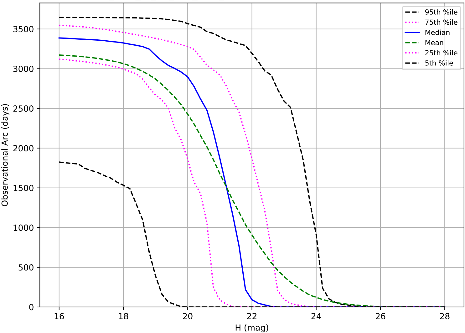
too_elab_r8_d3_griz_v3.4_10yrs: Observational Arc Length NEO
