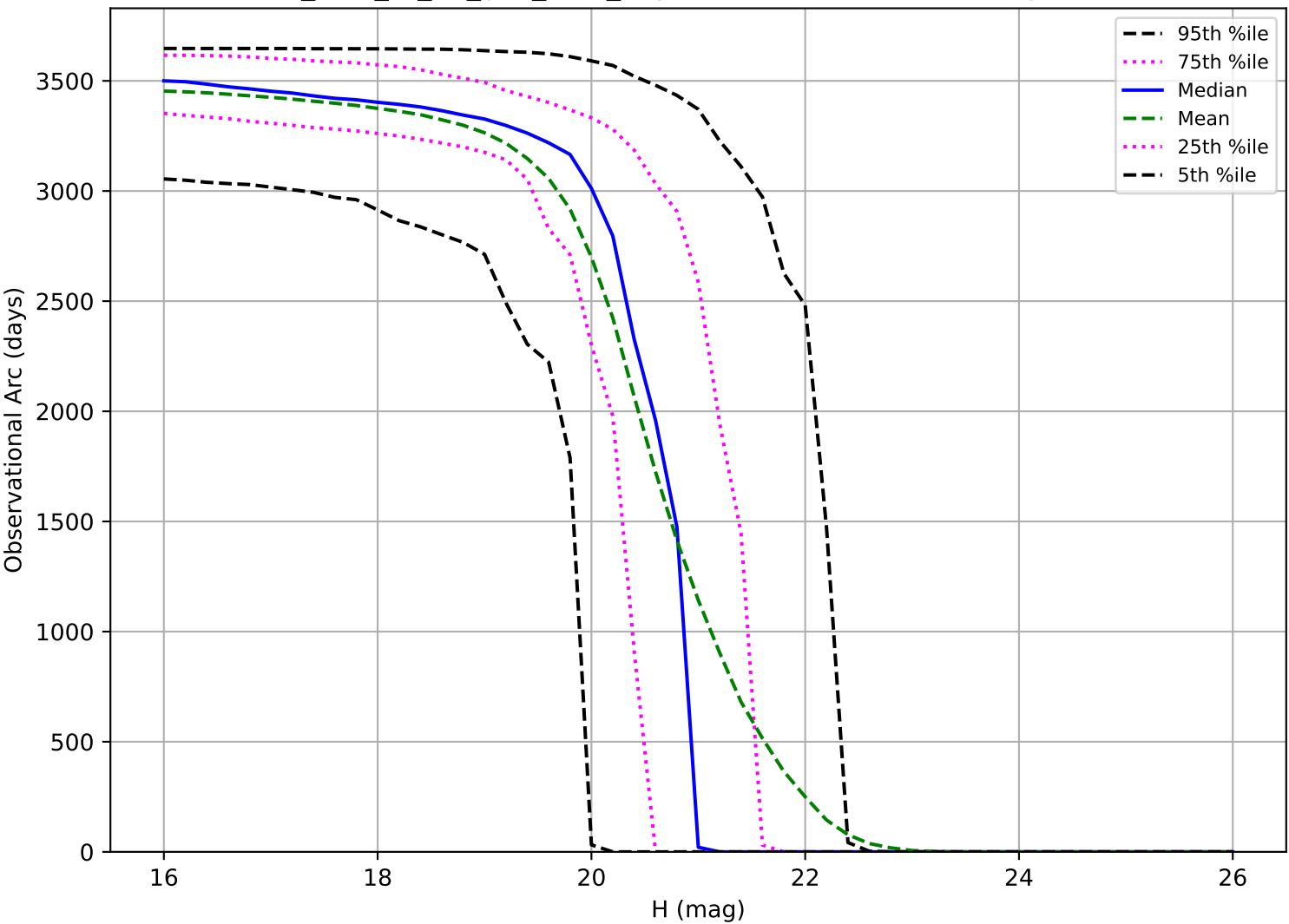
too_elab_r8_d3_griz_v3.4_10yrs: Observational Arc Length MBA
