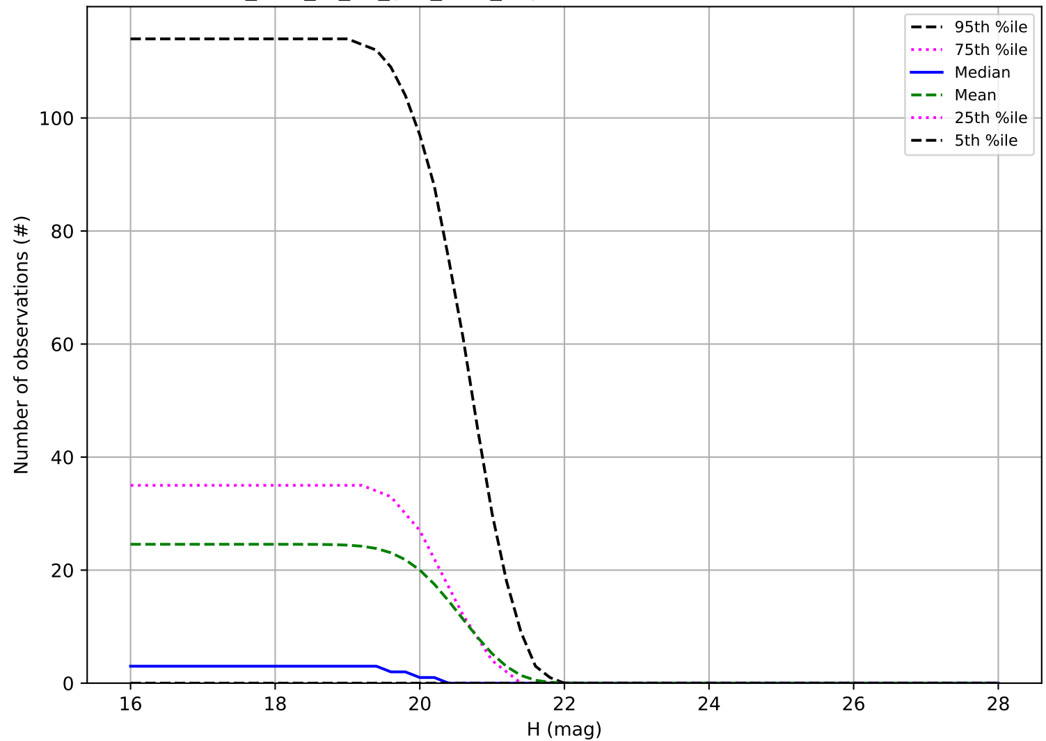
too_elab_r8_d3_griz_v3.4_10yrs: Number of observations Vatira
