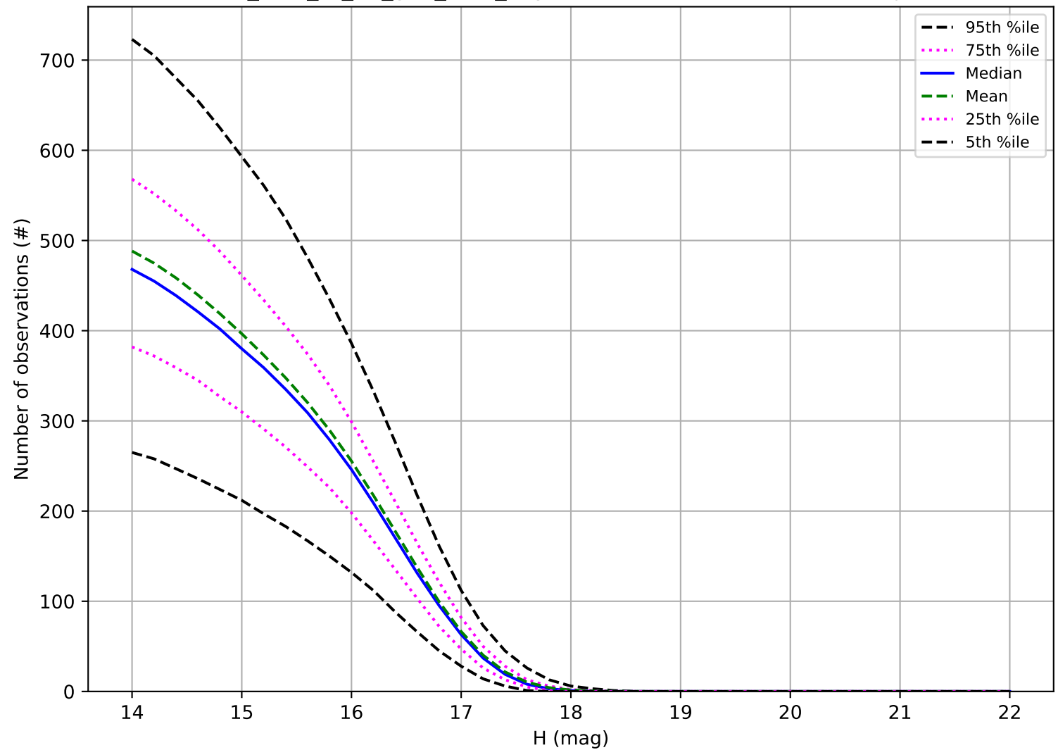
too_elab_r8_d3_griz_v3.4_10yrs: Number of observations Trojan
