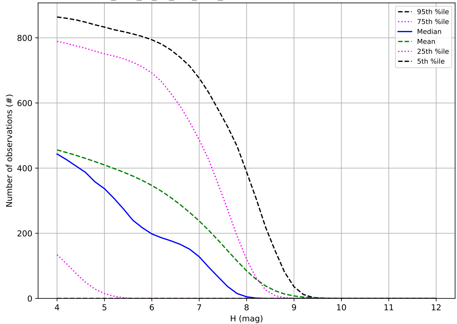
too_elab_r8_d3_griz_v3.4_10yrs: Number of observations TNO
