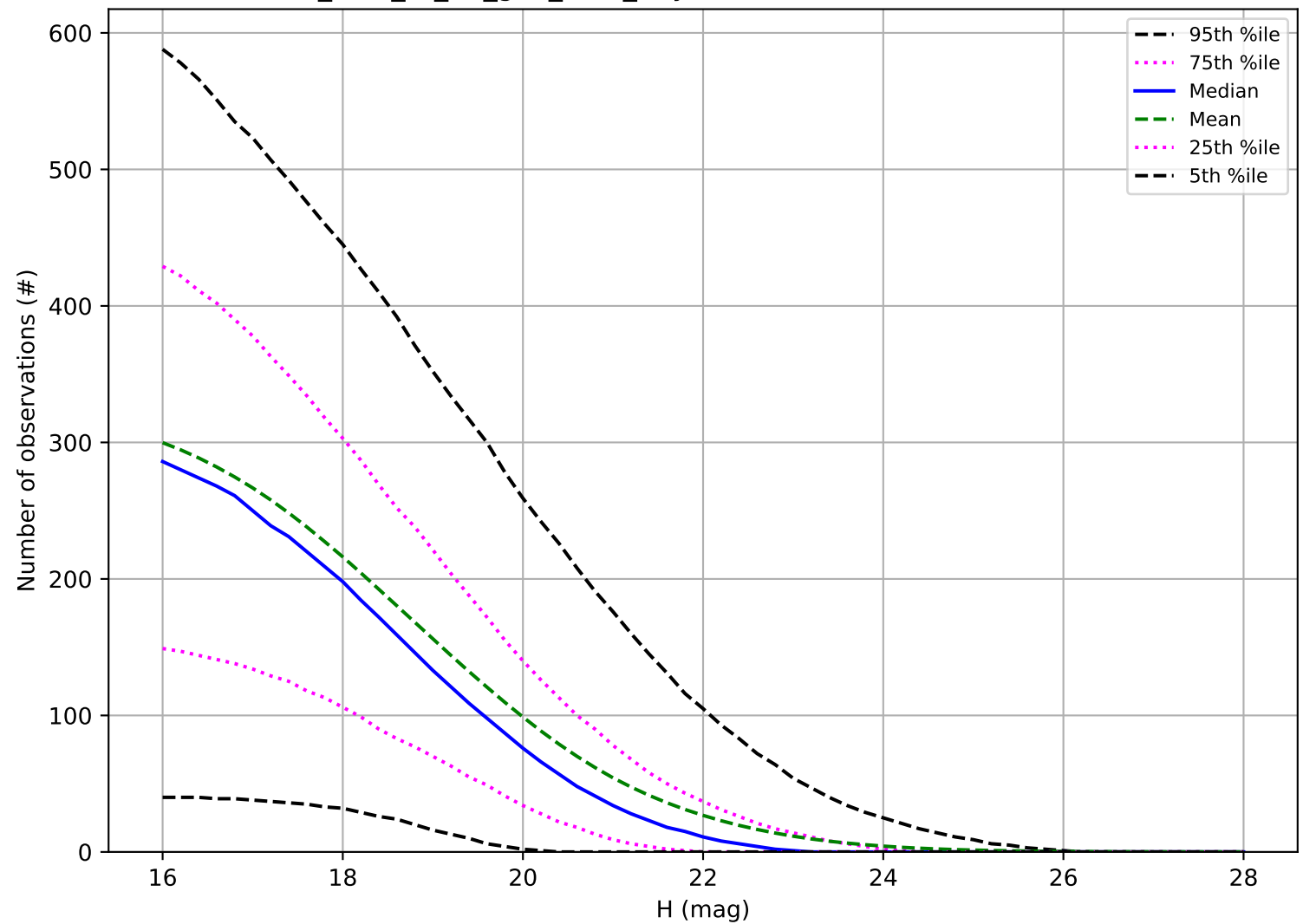
too_elab_r8_d3_griz_v3.4_10yrs: Number of observations PHA
