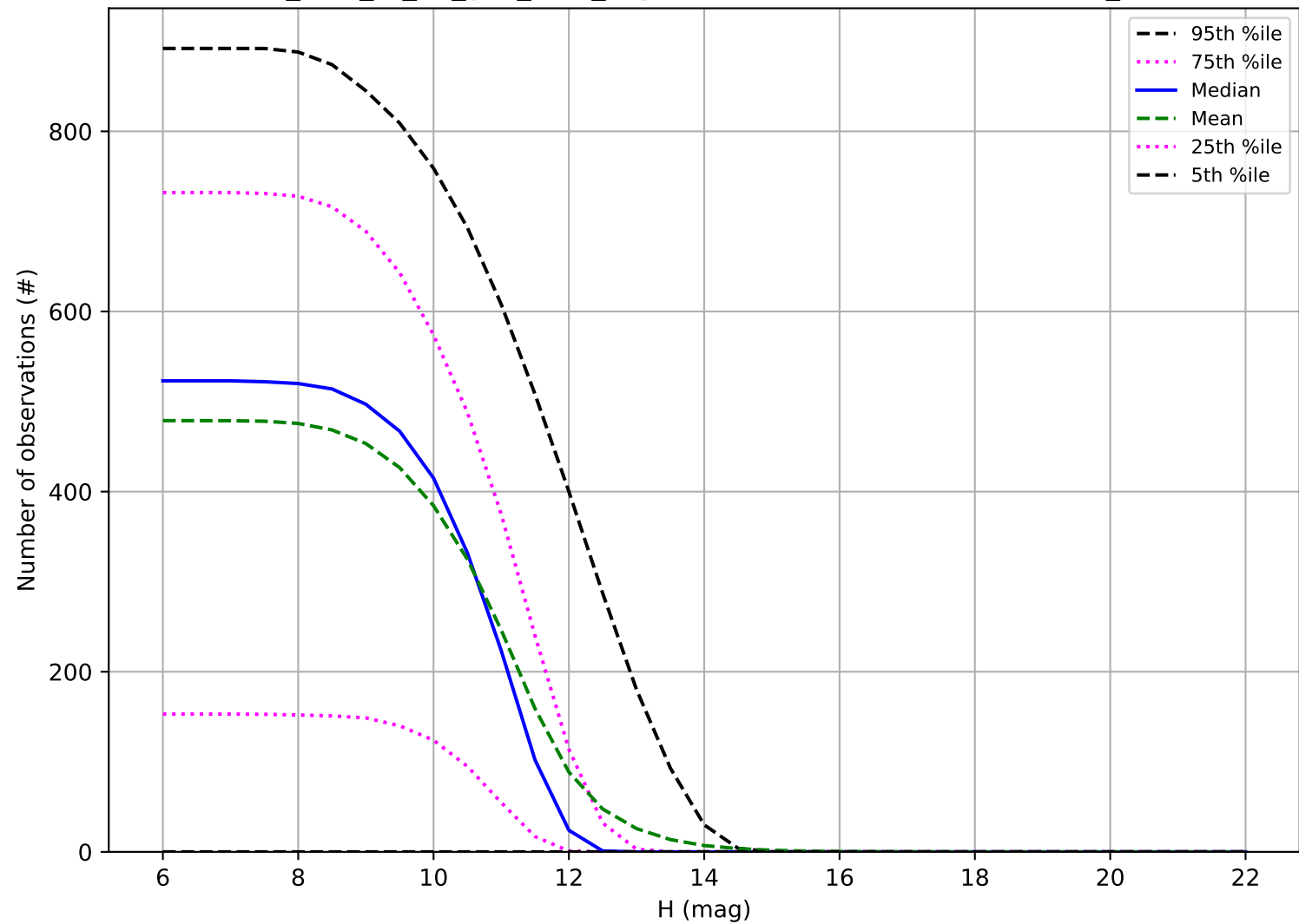
too_elab_r8_d3_griz_v3.4_10yrs: Number of observations OCC_r20
