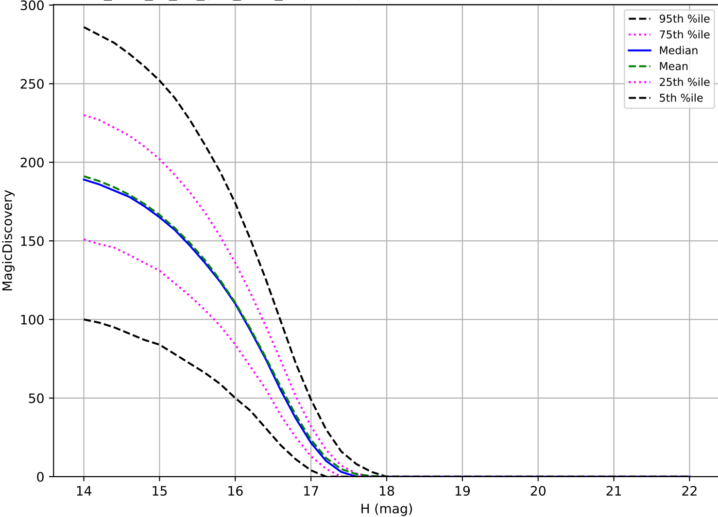
too_elab_r8_d3_griz_v3.4_10yrs: Trojan 6 detections in 60 nights detection loss
