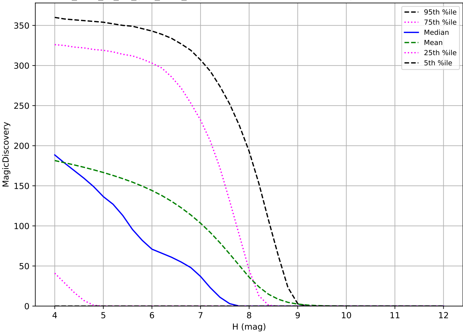
too_elab_r8_d3_griz_v3.4_10yrs: TNO 6 detections in 60 nights detection loss
