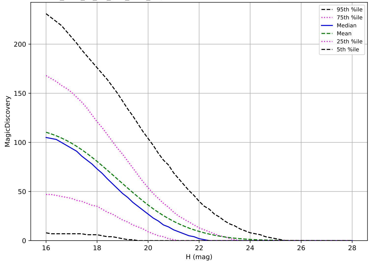
too_elab_r8_d3_griz_v3.4_10yrs: PHA 6 detections in 60 nights detection loss
