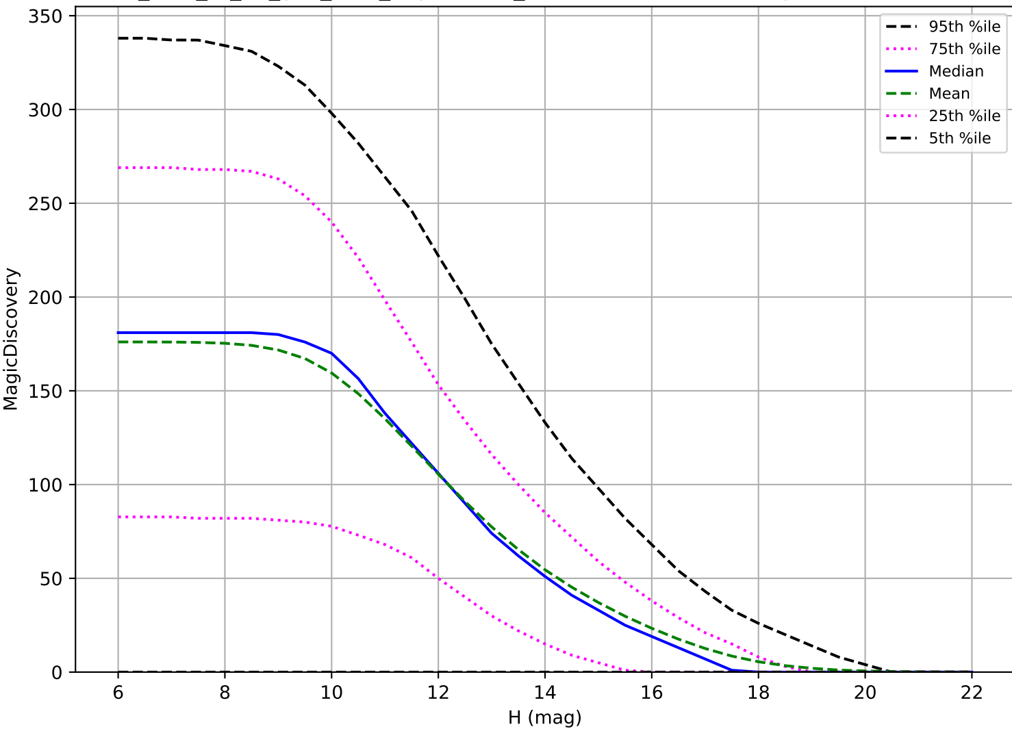
too_elab_r8_d3_griz_v3.4_10yrs: OCC_r5 6 detections in 60 nights detection loss
