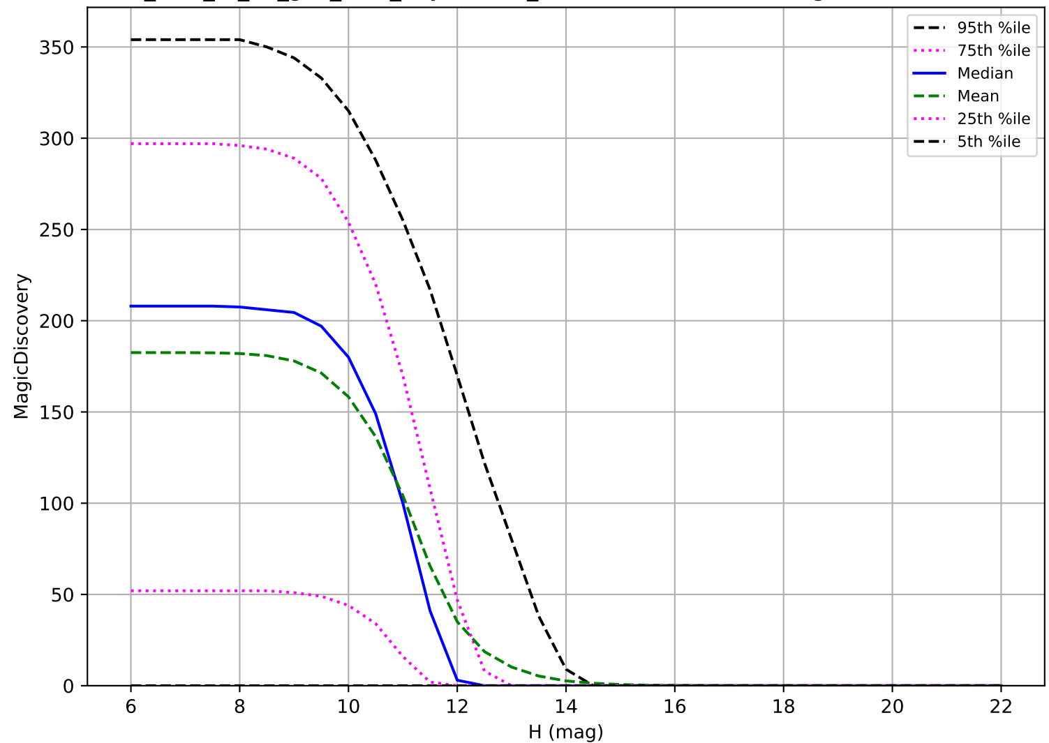
too_elab_r8_d3_griz_v3.4_10yrs: OCC_r20 6 detections in 60 nights detection loss
