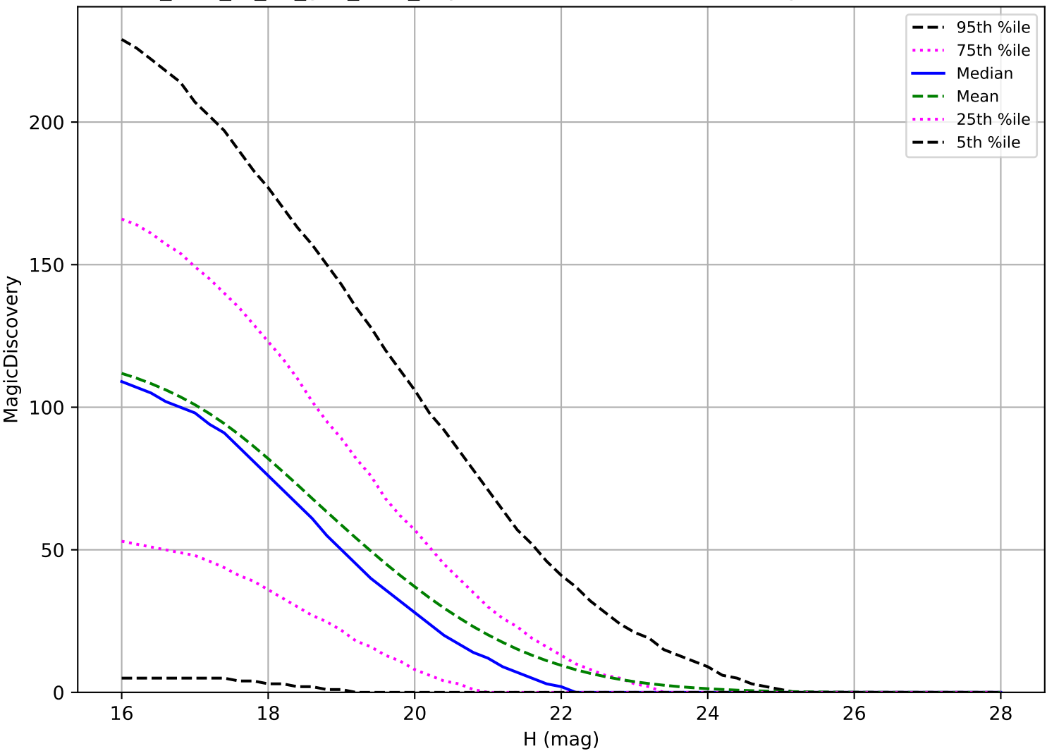
too_elab_r8_d3_griz_v3.4_10yrs: NEO 6 detections in 60 nights detection loss
