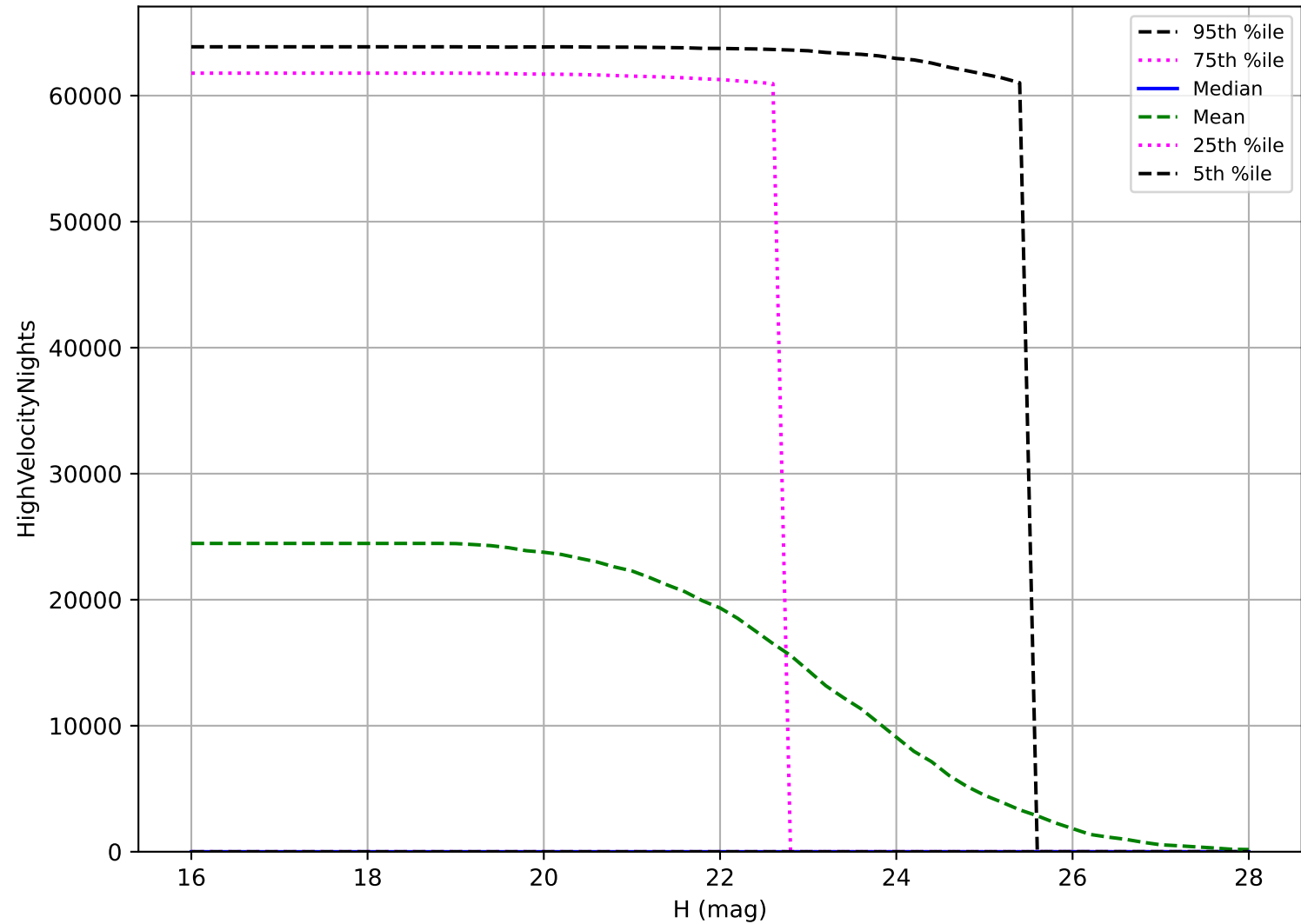
too_elab_r8_d3_griz_v3.4_10yrs: PHA High velocity pair detection loss
