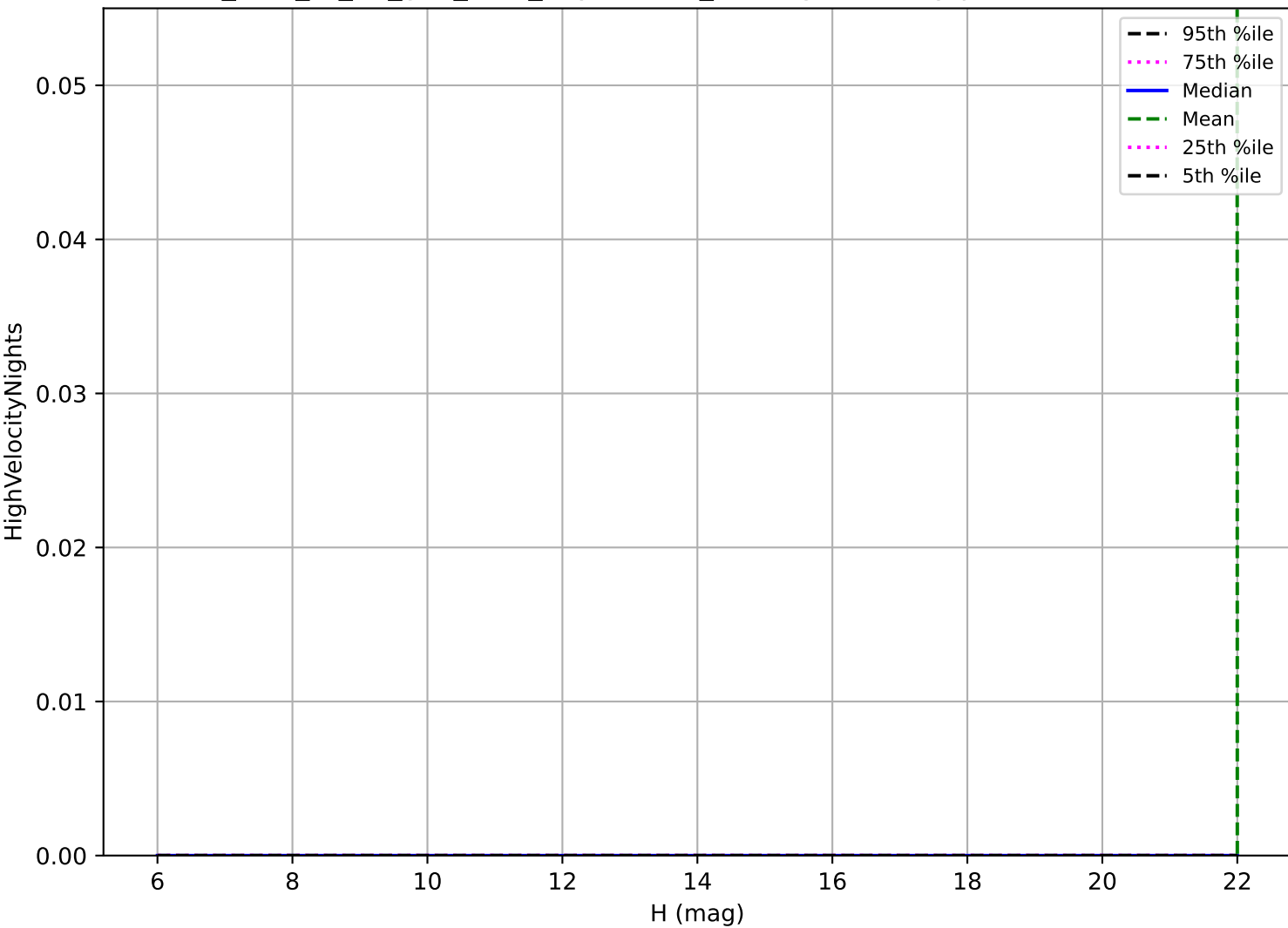
too_elab_r8_d3_griz_v3.4_10yrs: OCC_r20 High velocity pair detection loss
