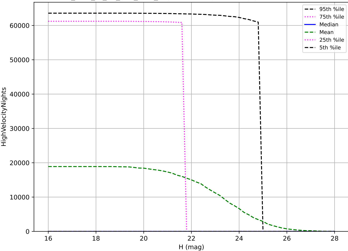
too_elab_r8_d3_griz_v3.4_10yrs: NEO High velocity pair detection loss
