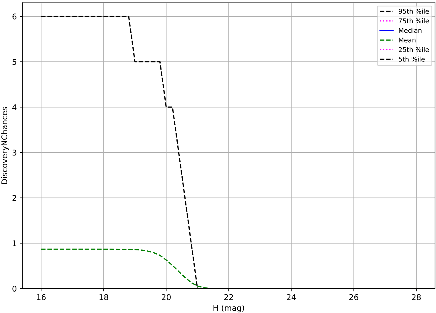
too_elab_r8_d3_griz_v3.4_10yrs: Vatira 3 pairs in 15 nights detection loss
