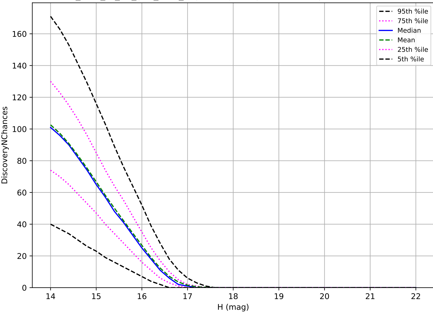
too_elab_r8_d3_griz_v3.4_10yrs: Trojan 3 pairs in 15 nights detection loss
