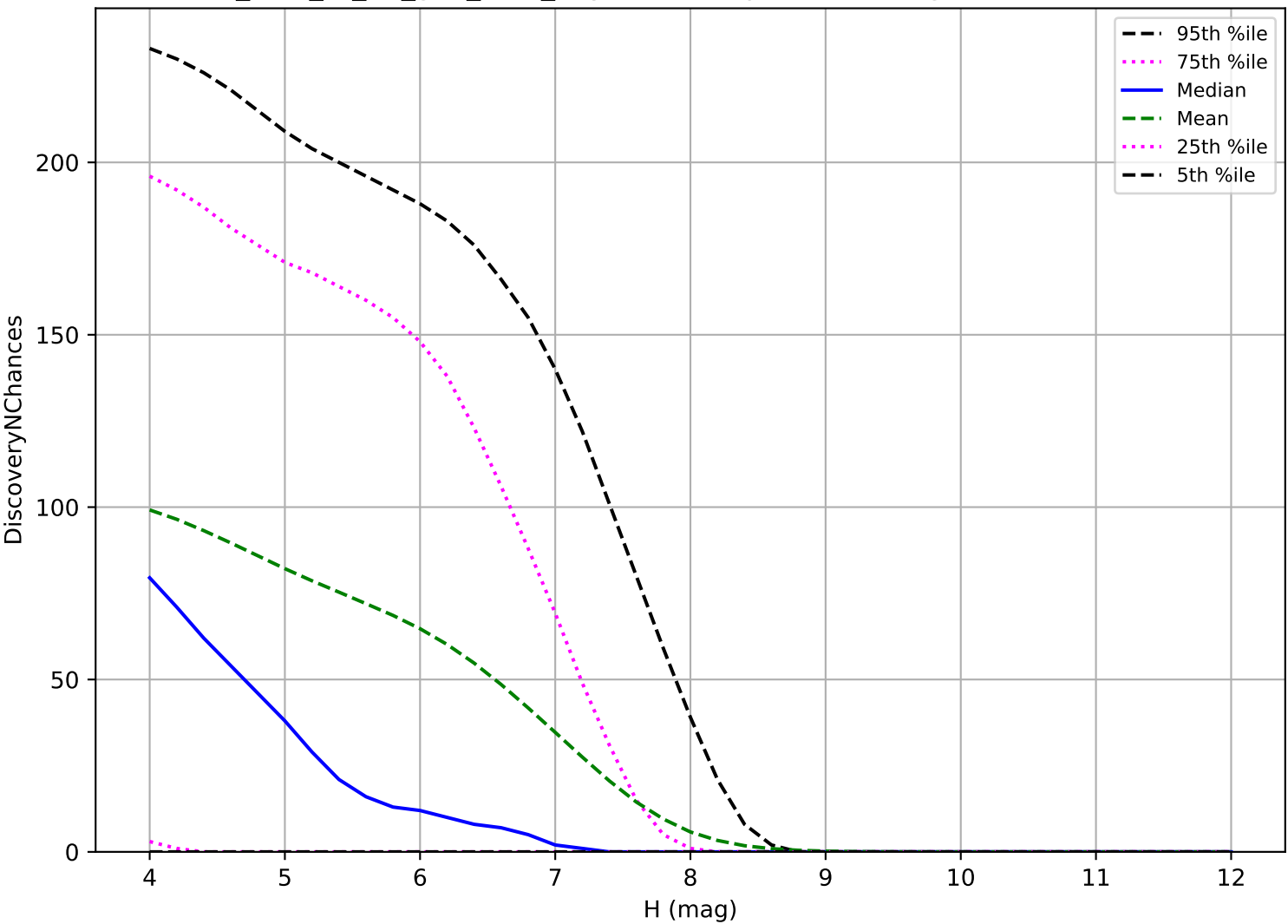
too_elab_r8_d3_griz_v3.4_10yrs: TNO 3 pairs in 15 nights detection loss
