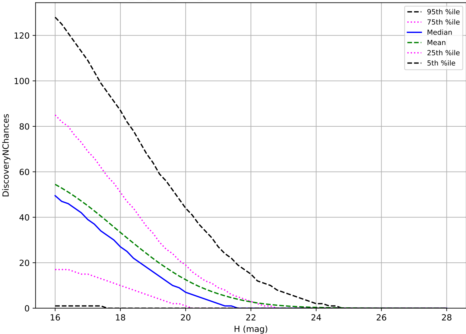
too_elab_r8_d3_griz_v3.4_10yrs: PHA 3 pairs in 15 nights detection loss
