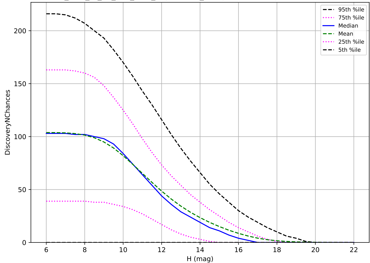
too_elab_r8_d3_griz_v3.4_10yrs: OCC_r5 3 pairs in 15 nights detection loss
