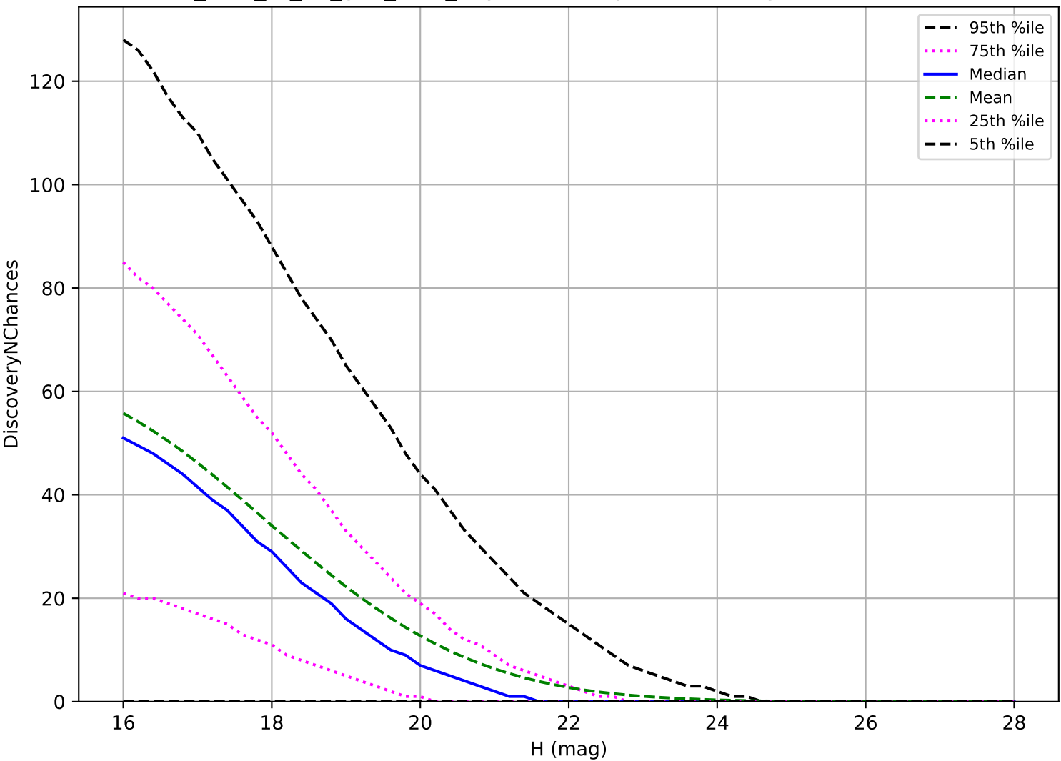
too_elab_r8_d3_griz_v3.4_10yrs: NEO 3 pairs in 15 nights detection loss
