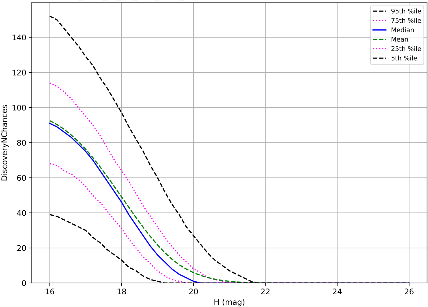
too_elab_r8_d3_griz_v3.4_10yrs: MBA 3 pairs in 15 nights detection loss
