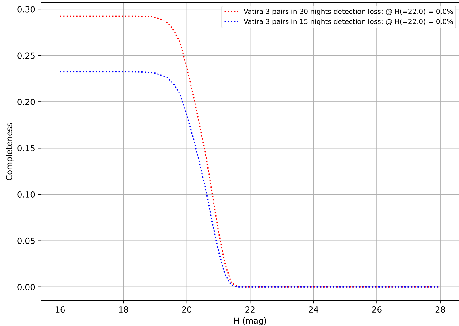
too_elab_r8_d3_griz_v3.4_10yrs: DifferentialCompleteness
