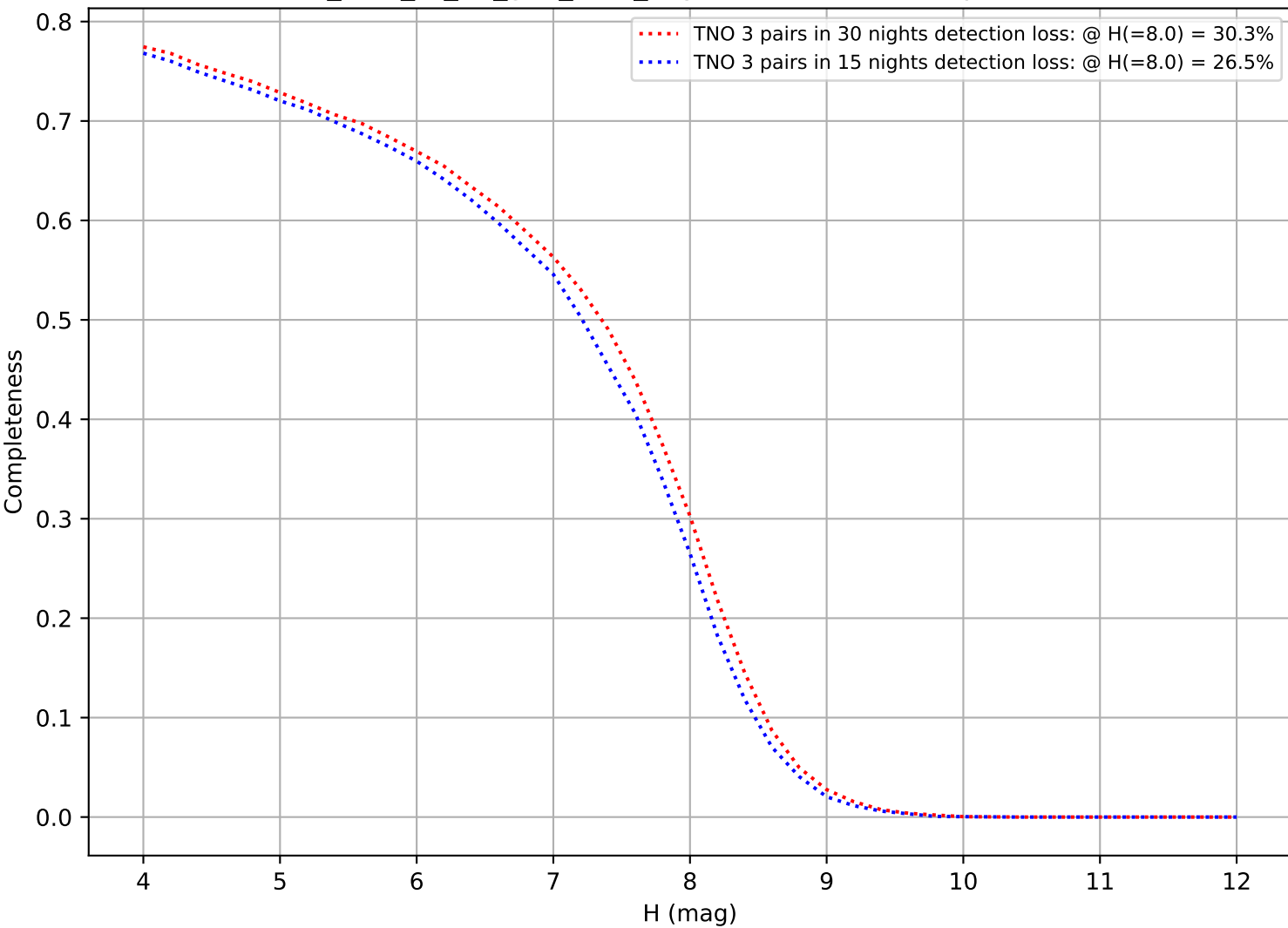
too_elab_r8_d3_griz_v3.4_10yrs: DifferentialCompleteness
