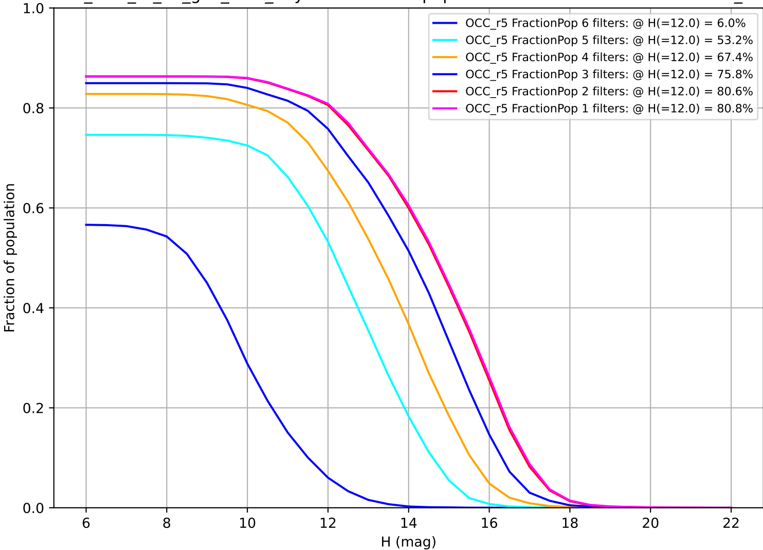
too_elab_r8_d3_griz_v3.4_10yrs: Fraction of population with colors in X filters OCC_r5
