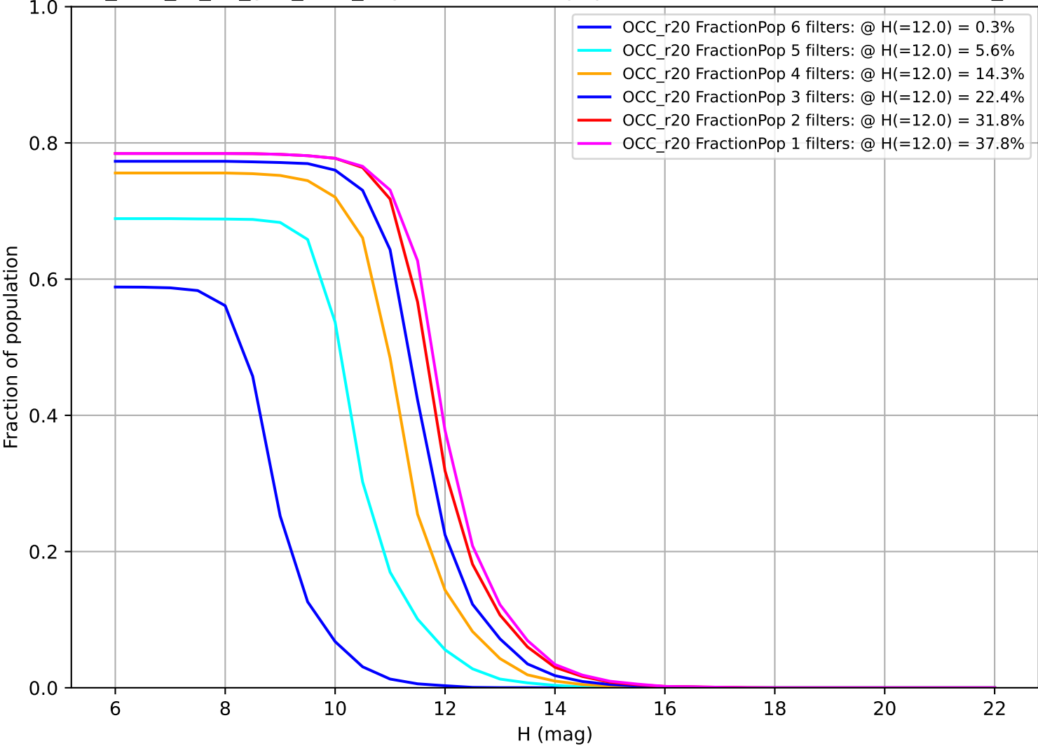
too_elab_r8_d3_griz_v3.4_10yrs: Fraction of population with colors in X filters OCC_r20
