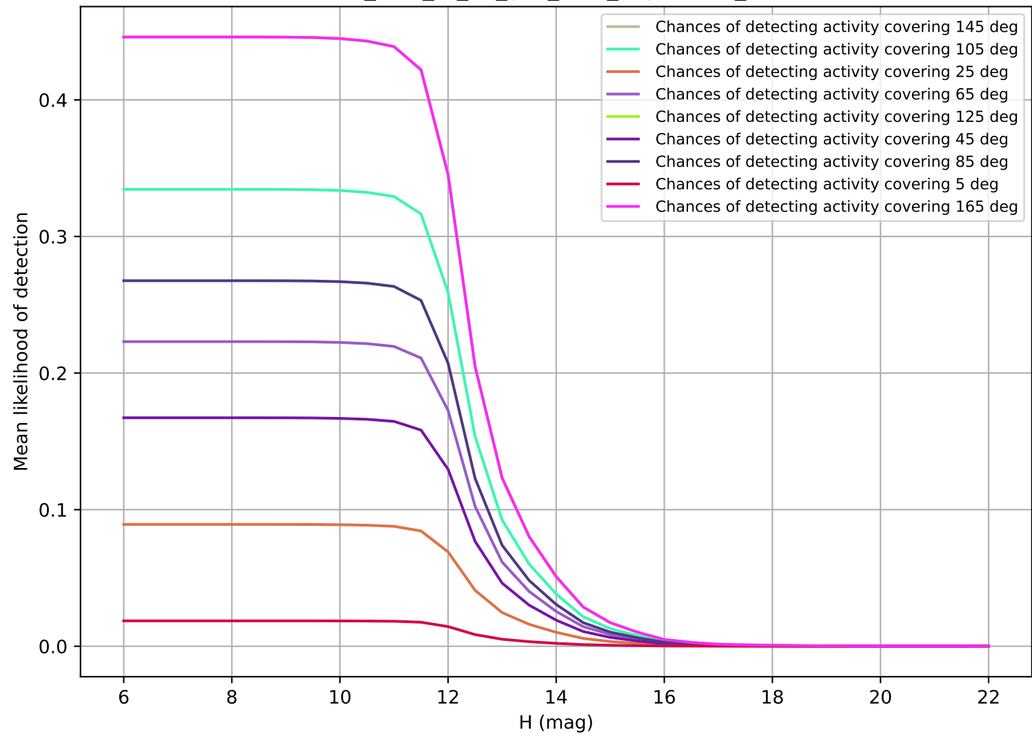
too_elab_r8_d3_griz_v3.4_10yrs OCC_r20
