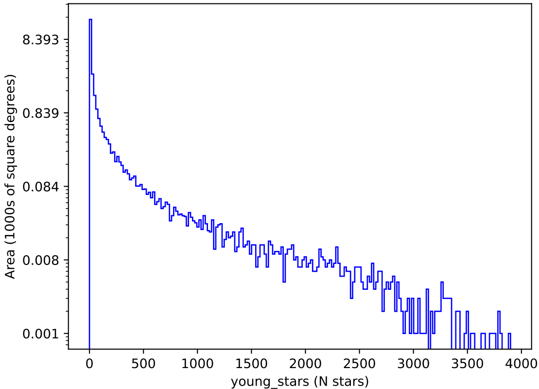
too_elab_r8_d3_griz_v3.4_10yrs : young_stars
