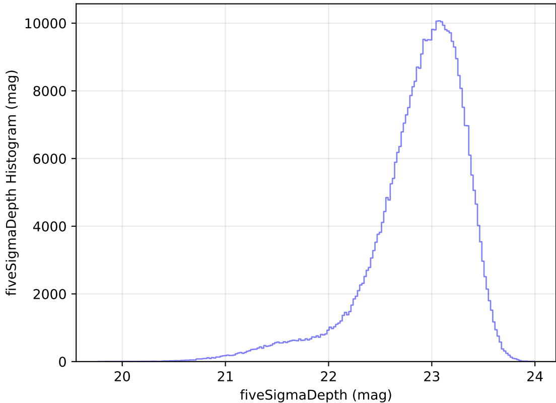
too_elab_r8_d3_griz_v3.4_10yrs z: fiveSigmaDepth Histogram
