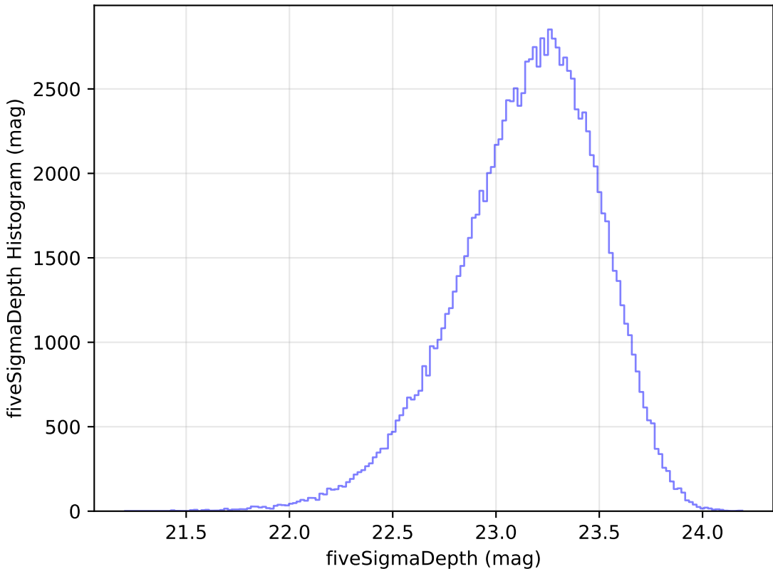
too_elab_r8_d3_griz_v3.4_10yrs u: fiveSigmaDepth Histogram
